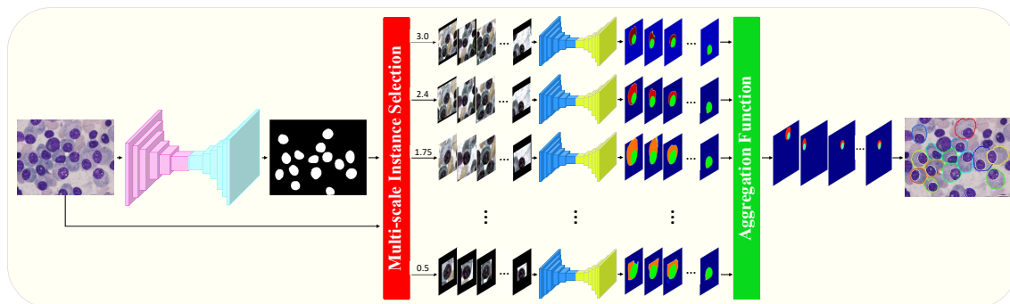
Figure 2: Proposed regional Attention Deeplabv3+ model for multiple myeloma plasma cells segmentation. The proposed method applies a U-net structure to learn the segmentation map for each nucleus instance then it utilizes multi-scale attention deeplabv3+ model to generate the segmentation mask for cytoplasm.
